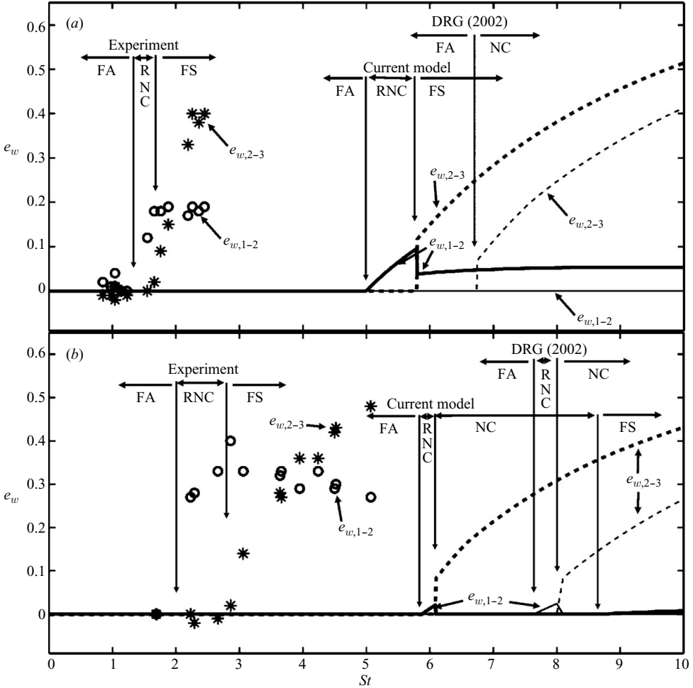
FIGURE 8. Wet restitution coefficient versus Stokes number for normal three-particle collisions with (a) 12 000 cP oil viscosity and stainless-steel particles (case h\mu_{cs.tk} in table 2, §4), and (b) 5120 cP oil viscosity and chrome-steel particles (case l\mu_{ss.tn} in table 2). The experimental results are compared against the modified theory of Davis et al. (2002) (DRG (2002)), represented by the thin lines, and the current model that uses the glass-transition pressure equal to 5.5 \times 10^8 Pa as a rebound point, represented by the thick lines.
