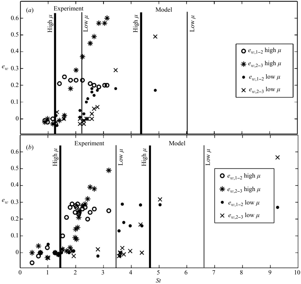
FIGURE 10. Effect of oil viscosity on the wet restitution coefficient for (a) chrome steel and thicker liquid layer (cases h\mu_{cs.tk} and \mu_{cs.tk} ), and (b) stainless steel and thinner liquid layer (cases h\mu_{ss.tn} and \mu_{ss.tn} ). The vertical solid lines demarcate St_{c,1-2} and show that this critical value for rebound shifts to higher values for both theory and experiment as the viscosity is decreased.
