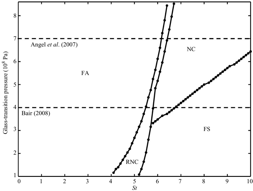
FIGURE 9. Regime map of glass-transition pressure versus St for 5120 cP viscosity oil, chrome-steel balls and thinner (case \mu_{cs,tn} in table 2, §4). The dashed lines demarcate the range of the glass-transition pressure for silicon oil that has been reported.
