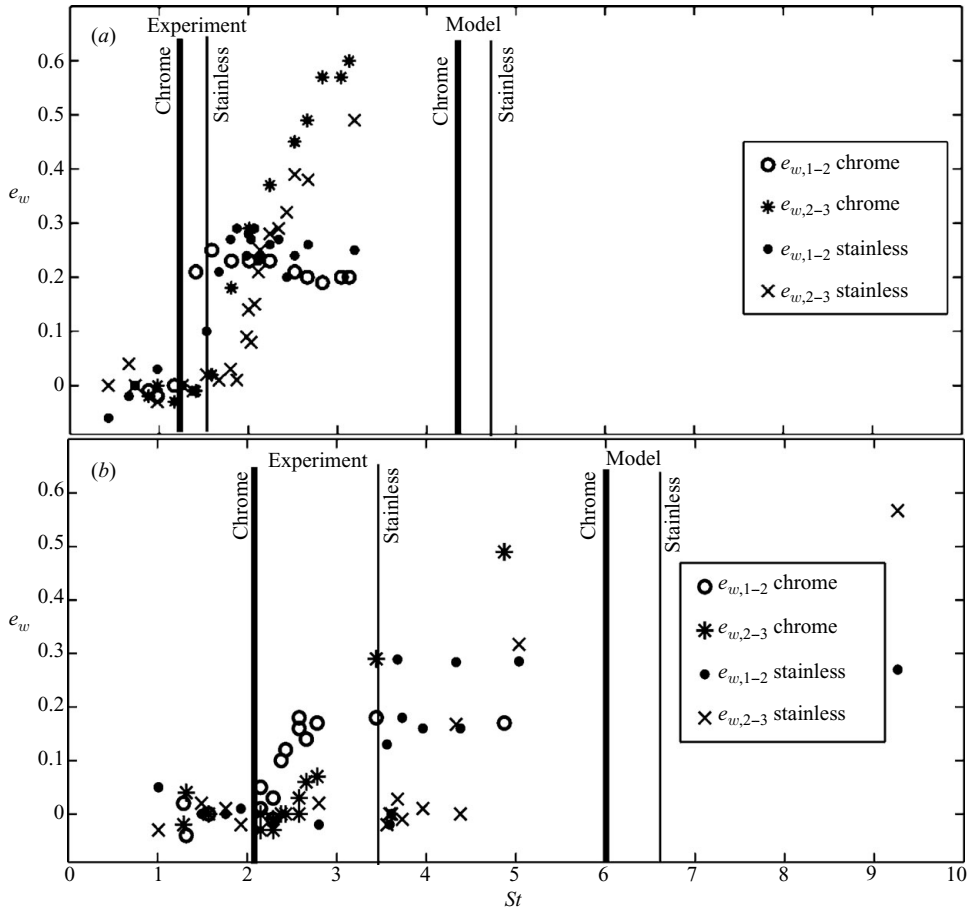
FIGURE 11. Effect of particle material on the wet restitution coefficient with (a) 12 000 cP and thicker liquid layer (cases h\mu_{cs.tk} and h\mu_{ss.tk} ), and (b) 5120 cP and thinner liquid layer (cases l\mu_{cs.tn} and l\mu_{ss.tn} ). The vertical solid lines demarcate St_{c,1-2} and show this critical value for rebound shifts to higher values for both theory and experiment as the dry restitution coefficient is decreased.
