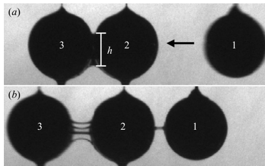
FIGURE 2. Snapshots of a three-particle wetted collision (a) just prior to collision and (b) after the collision using 12 000 cP oil viscosity and stainless-steel balls (case \mu_{ss\_tn} in table 2 below, see §4).
