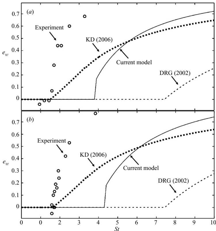
FIGURE 7. Wet restitution coefficient versus Stokes number for wet collisions between two particles with properties of (a) stainless-steel particles, 12 000 cP viscosity oil and 294 mm oil thickness and (b) chrome-steel particles, 5120 cP viscosity oil and 180 mm oil thickness. Comparisons are presented between experimental results and theories proposed by a modified form of Davis et al. (2002) (DRG (2002)), Kantak & Davis (2006) (KD (2006)) and the current model using a glass-transition pressure of 5.5 \times 10^8 Pa.
