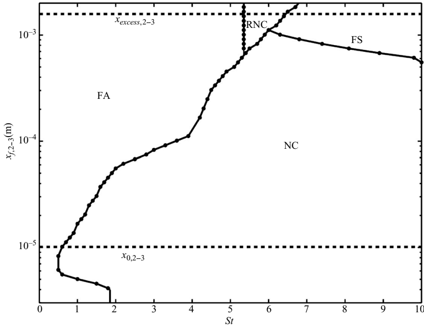
FIGURE 6. Predicted regime map as a function of x_{f,2-3} and St using parameters for 12000 cP oil and chrome-steel particles and thicker initial thickness (corresponding to case h\mu\_cs.tk in table 2, §4). Dashed horizontal lines represent x_{f,2-3} = x_{excess,2-3} and x_{f,2-3} = x_{0,2-3} . The model assumes that the oil undergoes a glass transition at 5.5 \times 10^8 Pa.
