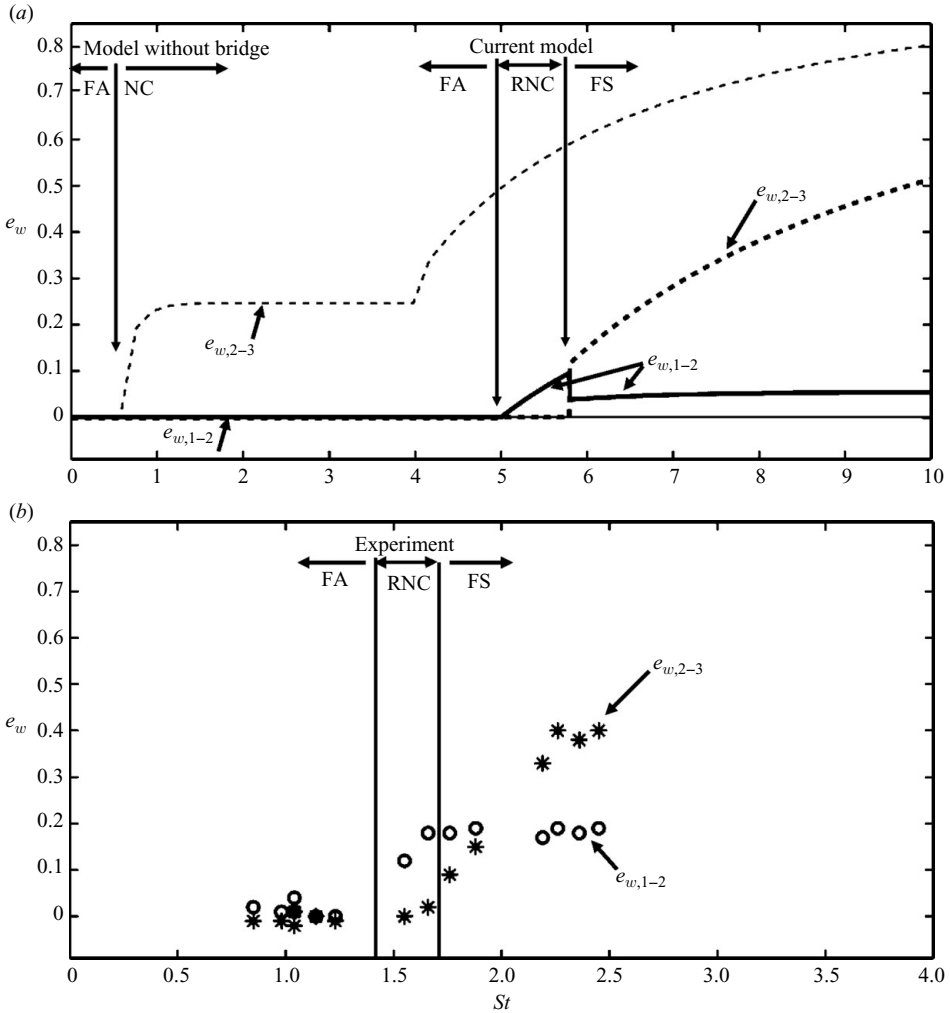
FIGURE 5. Comparisons of (a) theoretical predictions for e_w using the model without the bridge, x_{f,2-3} = x_{0,2-3} (thin) and the current model with x_{f,2-3} = x_{excess,2-3} (thick) and (b) experimental data using parameters for three-body collisions with 12 000 cP viscosity oil, chrome-steel particles and thick oil layer (case hp_cs.tk in table 2, §4). Both models assume that the oil undergoes a glass transition at 5.5 \times 10^8 Pa as a rebound criterion, which is the middle of the range of reported for silicon oil. Further details about the glass transition are discussed in §3.4.
