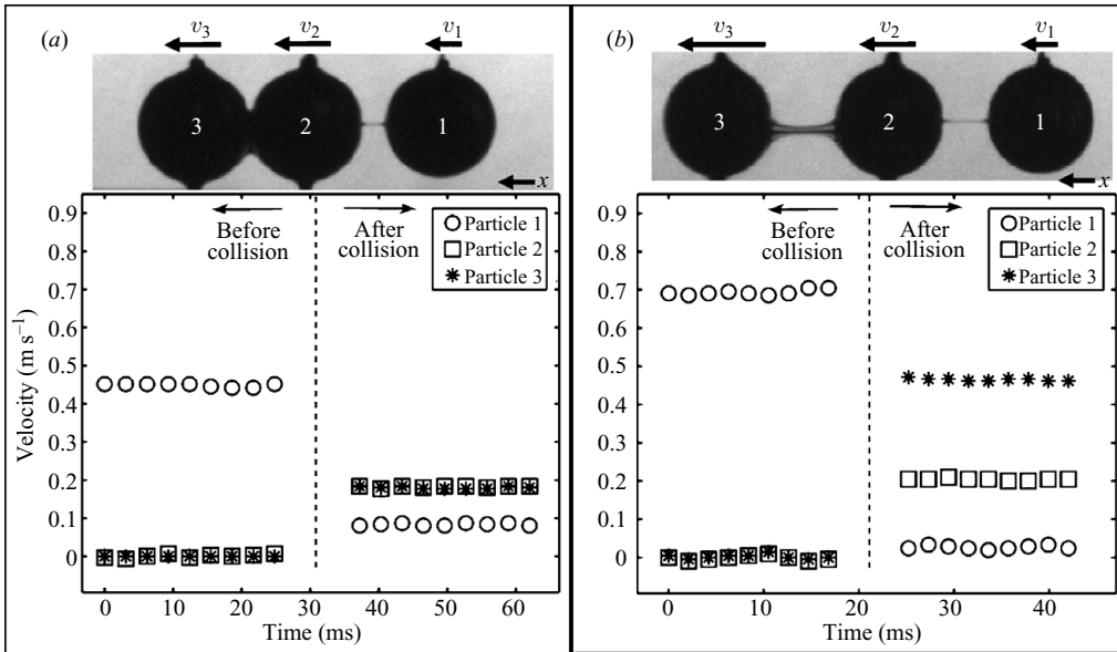
FIGURE 4. Snapshots after collision and corresponding velocity versus time plots for outcomes of (a) RNC and (b) FS using 12000 cP oil viscosity and stainless-steel ball material (case \mu_{ss\_tn} in table 2, §4). The initial velocity of particle 1 is from right to left.
